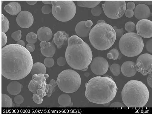
Figure 8: M789 powder by BÖHLER. PSD: 15-45 μm. SEM magnification: 600x.
